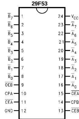
Pin Assignment for DIP
