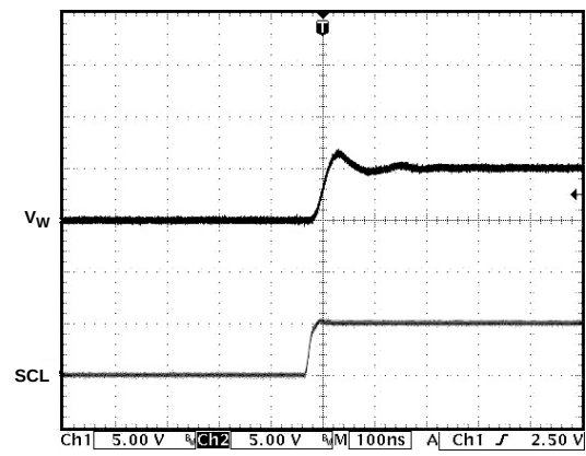
Figure 29. Large-Signal Settling Time
