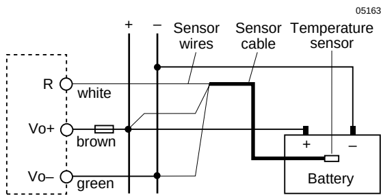
Fig. 6 Connection to a M, H, S, K, KP, LW or OK unit.
