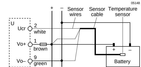
Fig. 4: Connection to the U unit.
