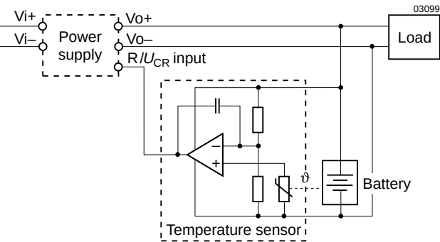
Fig. 2 Functional description
