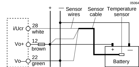
Fig. 3: Connection to the T unit.
