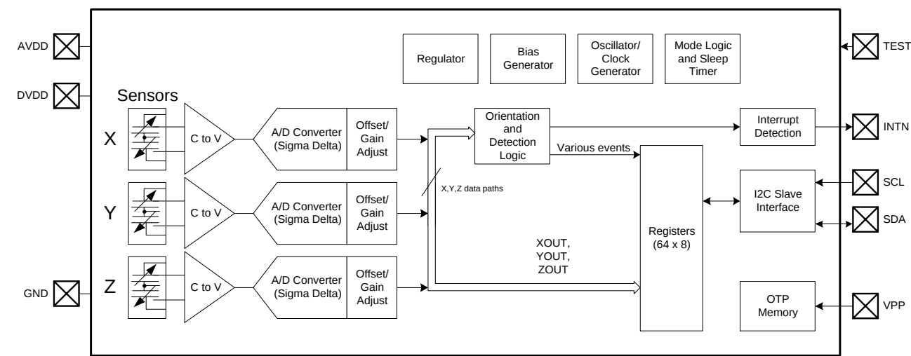
Figure 1. Block Diagram
