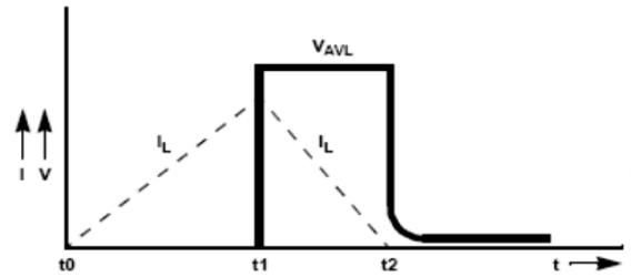
Figure 9. Unclamped Inductive Switching Test Circuit & Waveform
