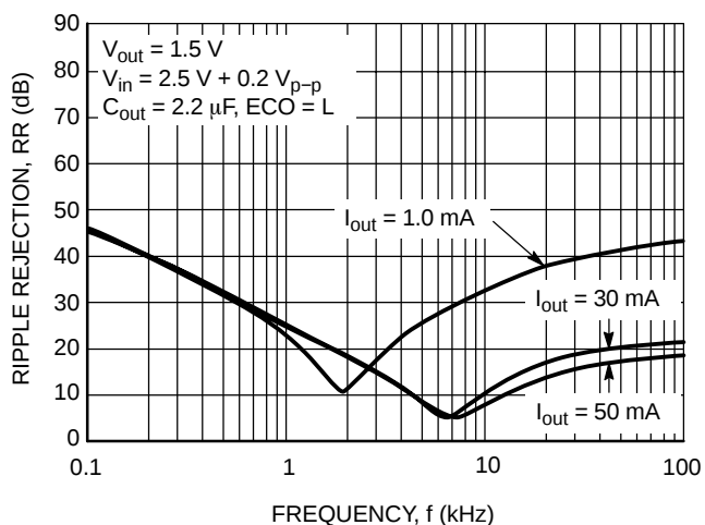
Figure 28. Ripple Rejection vs. Frequency
