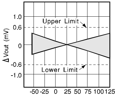
Temperature ^{\circ}C VRE205M
