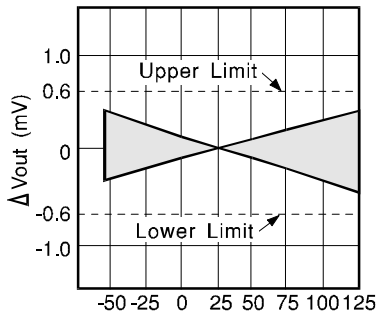
Temperature ^{\circ}\text{C} VRE204M
