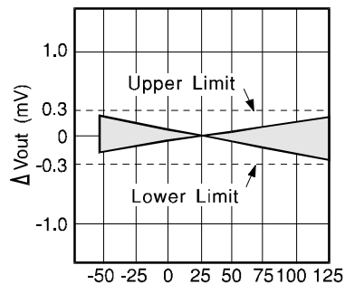
Temperature ^{\circ}\text{C} VRE204MA
