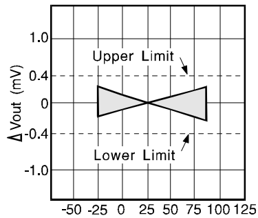
Temperature ^{\circ}\text{C} VRE204C
