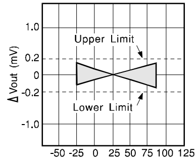
Temperature ^{\circ}\text{C} VRE204CA
