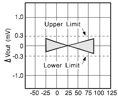
V_{OUT} vs. TEMPERATURE
