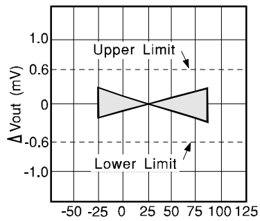
V_{OUT} vs. TEMPERATURE
