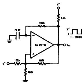
Squarewave Oscillator
