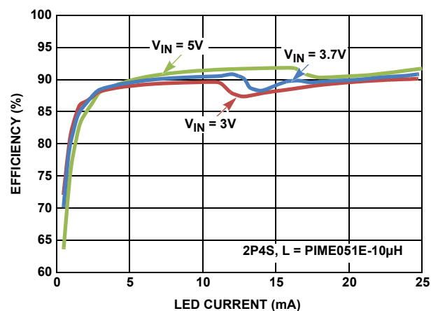
FIGURE 3. BOOST EFFICIENCY vs LED CURRENT (2P4S)
