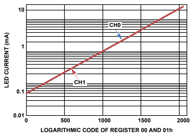
FIGURE 7. DIMMING Accuracy (11-BIT LOGARITHMIC MODE)
