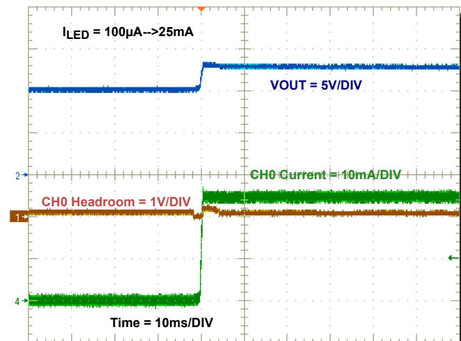
FIGURE 13. TRANSIENT RESPONSE (LED CURRENT CHANGES from 100μA to 25mA)
