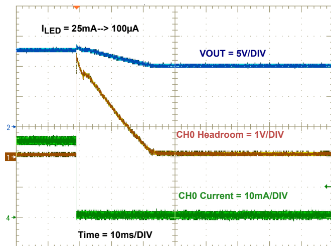
FIGURE 12. TRANSIENT RESPONSE (LED CURRENT CHANGES from 25mA to 100μA)
