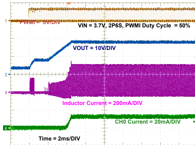
FIGURE 15. START-UP WAVEFORMS (50% BRIGHTNESS)
