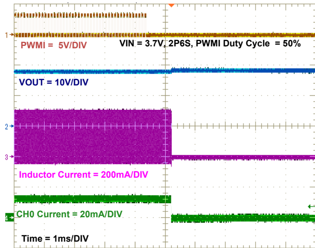
FIGURE 17. SHUTDOWN WAVEFORMS (50% BRIGHTNESS)
