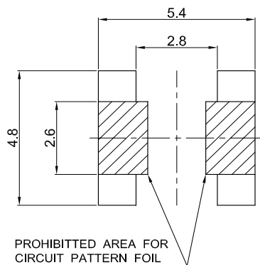
PRINTED CIRCUIT BOARD LAND DIMENSIONS (WHEN VIEWED FROM SWITCH MOUNTING SURFACE)
