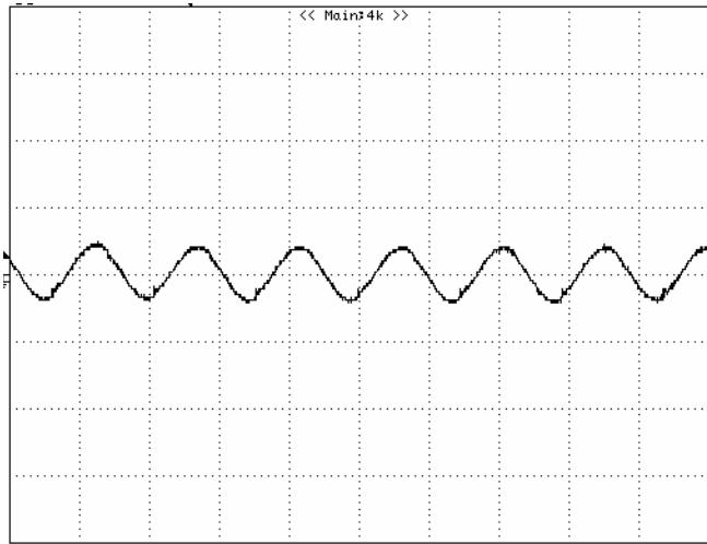
Figure 11: Input Terminal Ripple Current, i_c , at full rated output current and nominal input voltage with 12\mu\text{H} source impedance and 33\mu\text{F} electrolytic capacitor (100 mA/div, 2 \mu\text{s} /div).
