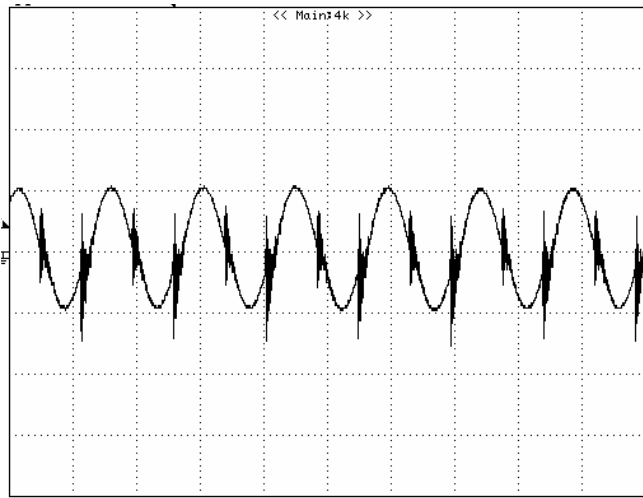
Figure 14: Output voltage ripple at nominal input voltage and rated load current ( I_o=25A ) (20 mV/div, 2 us/div) Load capacitance: 1 \mu F ceramic capacitor and 10 \mu F tantalum capacitor. Bandwidth: 20 MHz. Scope measurements should be made using a BNC cable (length shorter than 20 inches). Position the load between 51 mm to 76 mm (2 inches to 3 inches) from the module.
