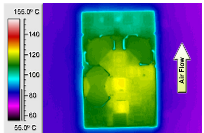
Figure 12: Thermal plot of converter at 8.1 amp load current with 85°C air flowing at the rate of 200 LFM. Air is flowing across the converter from input to output (48V input).
