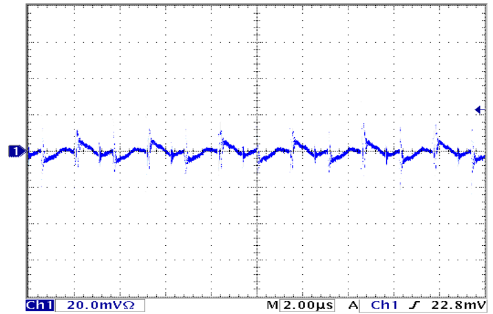
Figure 20: Output voltage ripple at nominal input voltage and rated load current (20 mV/div). Load capacitance: 1 \mu F ceramic capacitor and 10 \mu F tantalum capacitor. Bandwidth: 20 MHz. See Figure 17.
