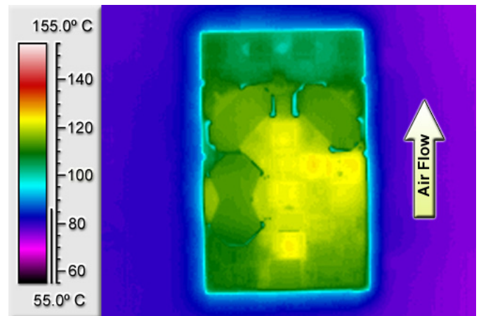
Figure 10: Thermal plot of converter at 8.33 amp load current with 85°C air flowing at the rate of 200 LFM. Air is flowing across the converter from input to output (24V input).
