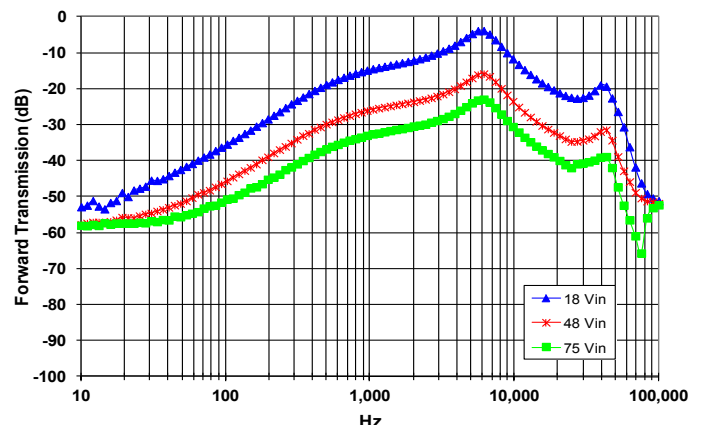
Figure 24: Magnitude of incremental forward transmission ( FT = v_{out}/v_{in} ) for minimum, nominal, and maximum input voltage at full rated power.
