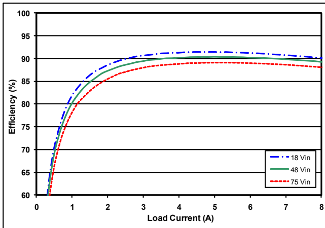
Figure 1: Efficiency at nominal output voltage vs. load current for 18V, 48V and 75V input at 25°C.
