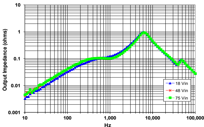
Figure 23: Magnitude of incremental output impedance ( Z_{out} = v_{out}/i_{out} ) for minimum, nominal, and maximum input voltage at full rated power.
