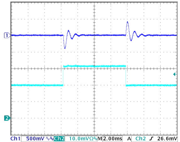
Figure 16: Output voltage response to step-change in load current (50%-75%-50% of Iout(max); dI/dt = 5A/μs). Load cap: 470μF, 30 mW ESR tantalum cap and 1μF ceramic cap. Ch 1: Vout (500mV/div), Ch 2: Iout (2A/div).
