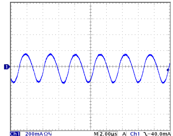
Figure 18: Input Terminal Ripple Current, I C , at full rated output current and nominal input voltage with 10μH source impedance and 47μF electrolytic capacitor (200 mA/div). See Figure 17.
