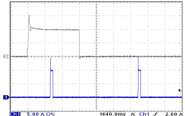
Figure 22: Load current (5A/div) as a function of time when the converter attempts to turn on into a 10 mW short circuit. Top trace (40ms/div) is an expansion of the on-time portion of the bottom trace.
