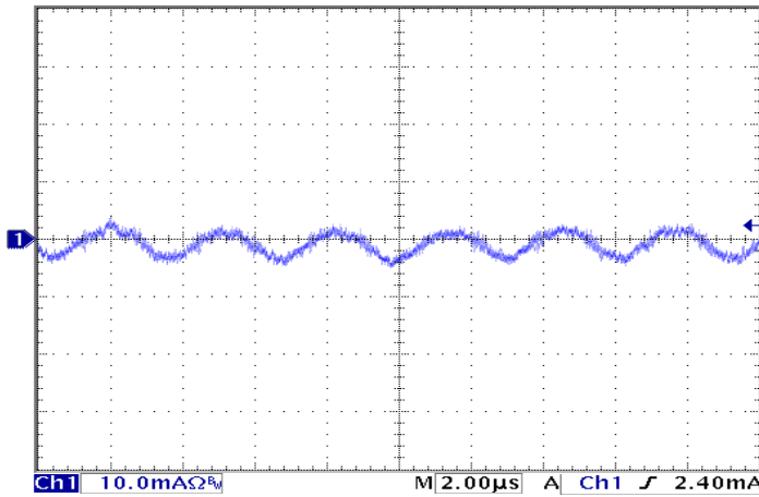
Figure 19: Input reflected ripple current, is, through a 10 \mu H source inductor at nominal input voltage and rated load current (10 mA/div). See Figure 17.
