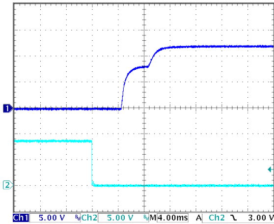
Figure 13: Turn-on transient at full load (resistive load) (4 ms/div). Input voltage pre-applied. Ch 1: Vout (5V/div). Ch 2: ON/OFF input (5V/div).
