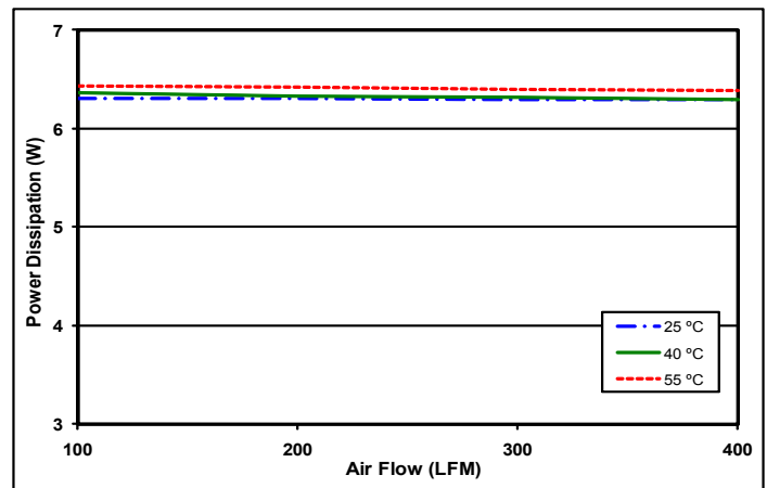
Figure 4: Power dissipation at nominal output voltage and 60% rated power vs. airflow rate for ambient air temperatures of 25°C, 40°C, and 55°C (nominal input voltage, 48V input).
