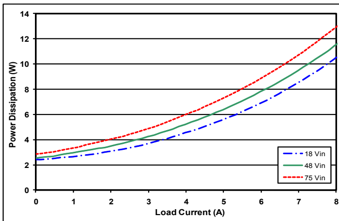
Figure 3: Power dissipation at nominal output voltage vs. load current for 18V, 48V and 75V input at 25°C.
