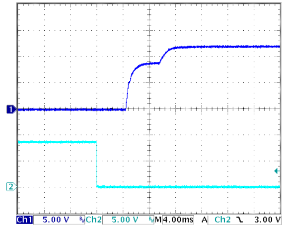
Figure 14: Turn-on transient at zero load (4 ms/div). Ch 1: Vout (5V/div). Ch 2: ON/OFF input (5V/div).
