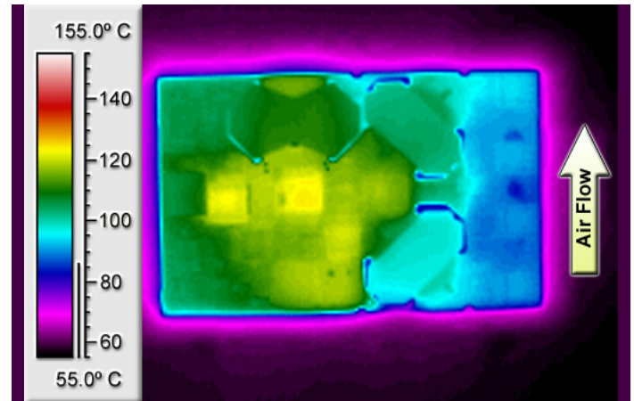
Figure 8: Thermal plot of converter at 8.1 amp load current with 55°C air flowing at the rate of 200 LFM. Air is flowing across the converter sideways from pin 3 to pin 1 (48V input).
