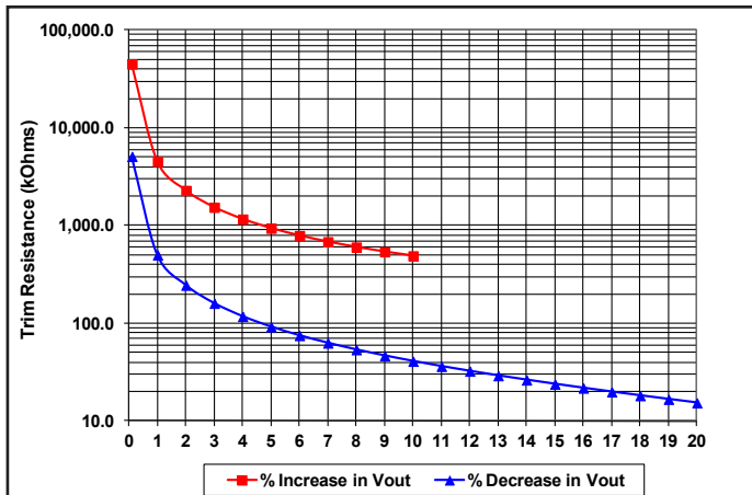
Figure C: Trim Graph
