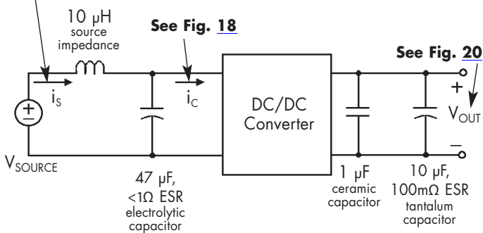
Figure 17: Test set-up diagram showing measurement points for Input Terminal Ripple Current (Figure 18), Input Reflected Ripple Current (Figure 19) and Output Voltage Ripple (Figure 20).
