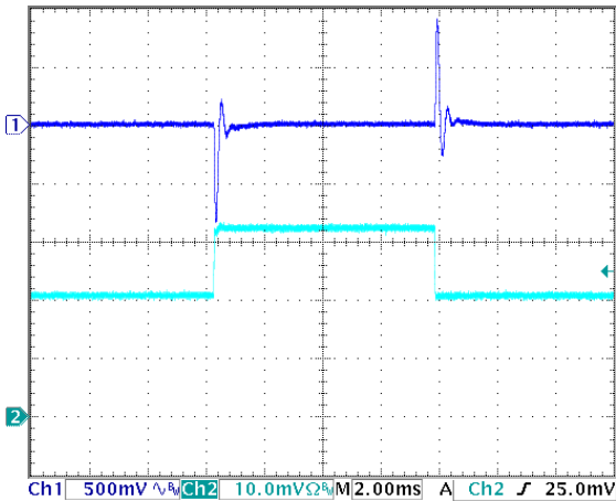
Figure 15: Output voltage response to step-change in load current (50%-75%-50% of Iout(max); dI/dt = 0.1A/μs). Load cap: 10μF, 100 mW ESR tantalum cap and 1μF ceramic cap. Ch 1: Vout (500mV/div), Ch 2: Iout (2A/div).
