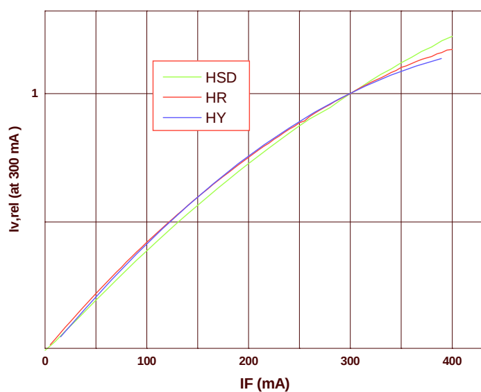
I_F - I_{v, rel} characteristic
