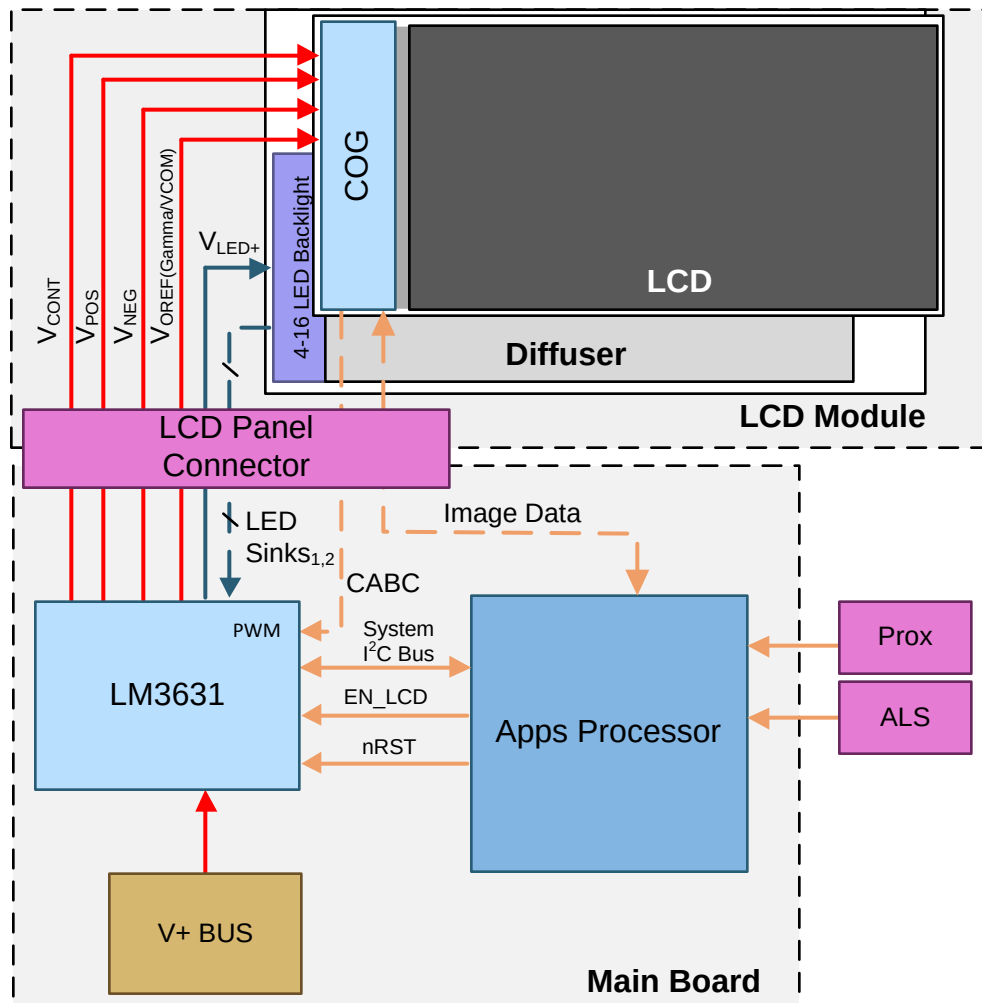
Figure 38. System Example
