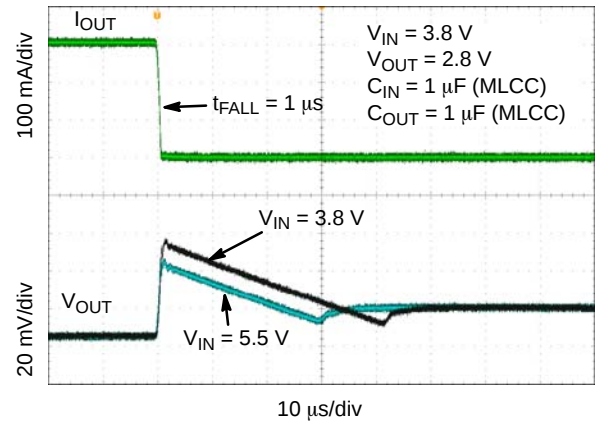
Figure 42. Load Transient Response – Falling Edge, V_{OUT} = 2.8 V , I_{OUT} = 1 mA to 300 mA, V_{IN} = 3.8 V , 5.5 V
