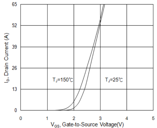
Fig.8 Transfer Characteristics
