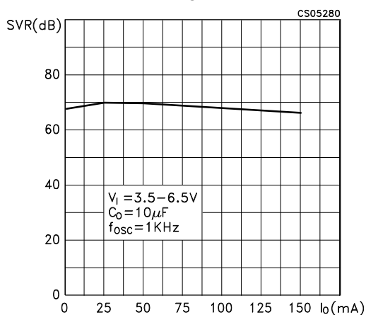
Figure 9. Supply voltage rejection vs. output current ( C_o = 10\mu\text{F} )
