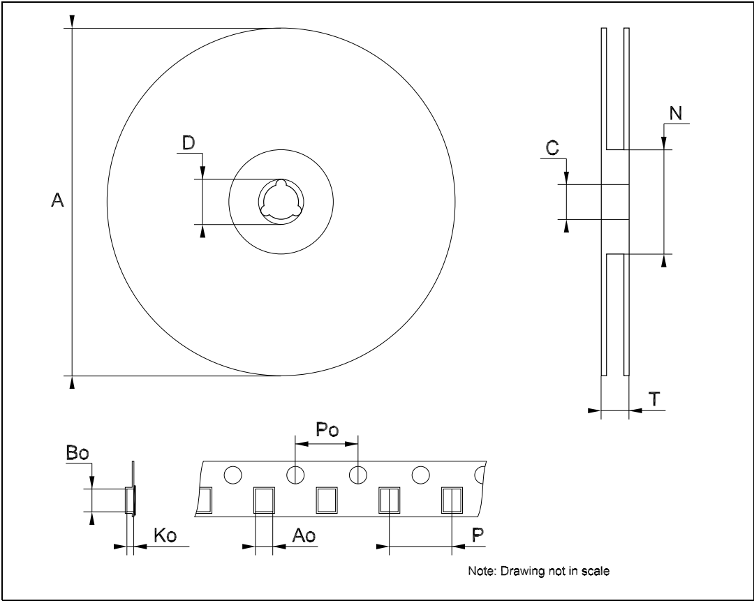
Figure 20. Tape and reel SOT23-5L outline
