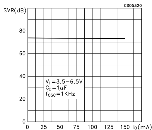
Figure 10. Supply voltage rejection vs. output current ( C_o = 1\mu\text{F} )
