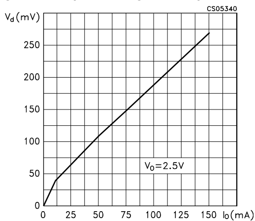
Figure 5. Dropout voltage vs. output current
