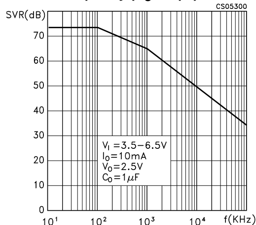
Figure 12. Supply voltage rejection vs. frequency ( C_o = 1\mu\text{F} )
