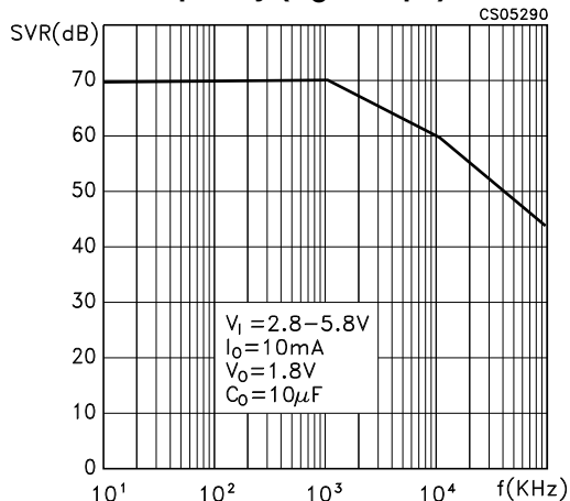
Figure 11. Supply voltage rejection vs. frequency ( C_o = 10\mu\text{F} )
