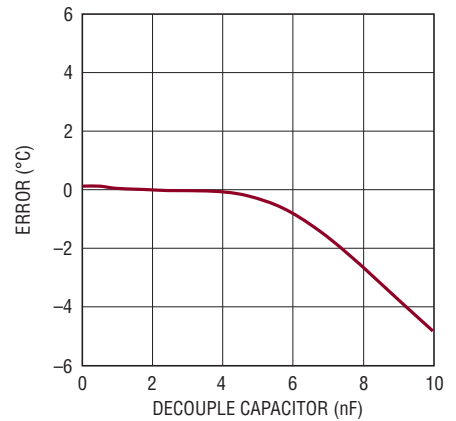
Remote Temperature Error vs C_{\text{DECOUPLE}} (Between D^+ and D^- )
