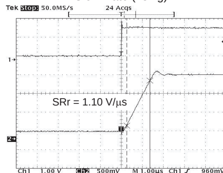
Figure 20 HA1630S07 Slew Rate (rising)
