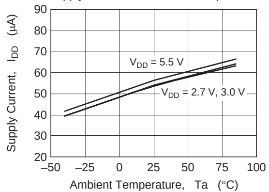
Figure 2 HA1630S07 Supply Current vs. Ambient Temperature
