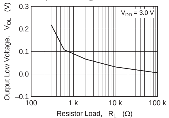
Figure 4 HA1630S07 Output Low Voltage vs. Resistor Load
