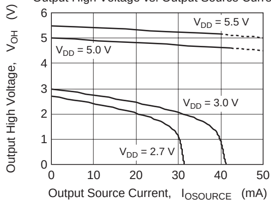
Figure 5 HA1630S07 Output High Voltage vs. Output Source Current
