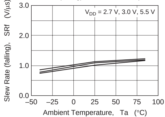
Figure 22 HA1630S07 Slew Rate (falling) vs. Ambient Temperature
