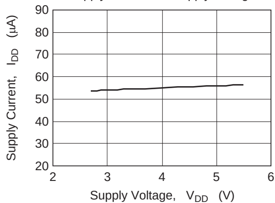
Figure 1 HA1630S07 Supply Current vs. Supply Voltage
