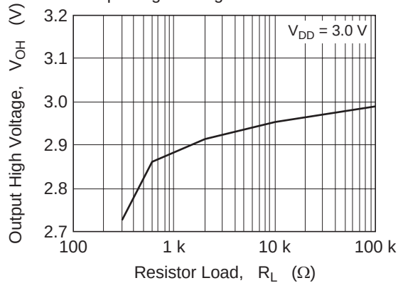
Figure 3 HA1630S07 Output High Voltage vs. Resistor Load
