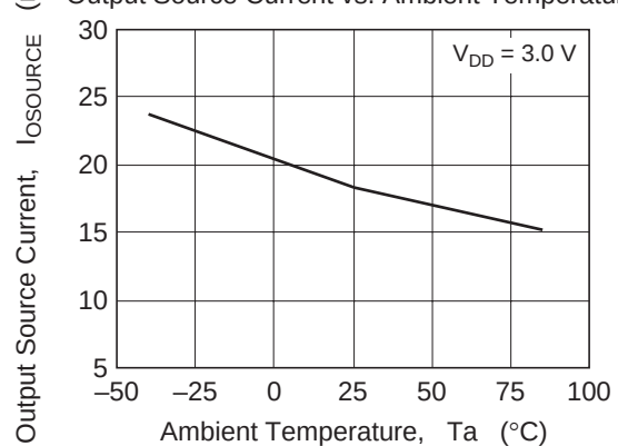
Figure 6 HA1630S07 Output Source Current vs. Ambient Temperature
