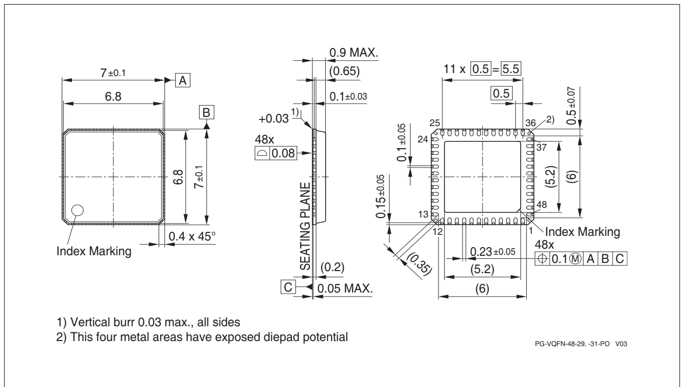
Figure 63 PG-VQFN-48-31
