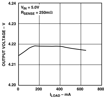
TPC 22. Charger V OUT vs. I LOAD (V IN = 5.0 V)
