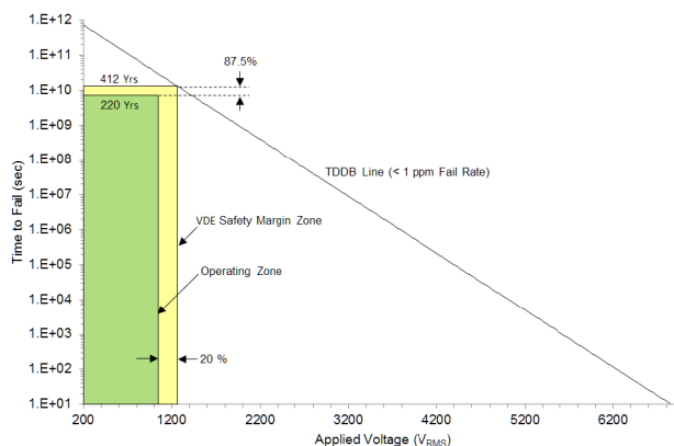
Figure 9-4. Insulation Lifetime Projection Data
