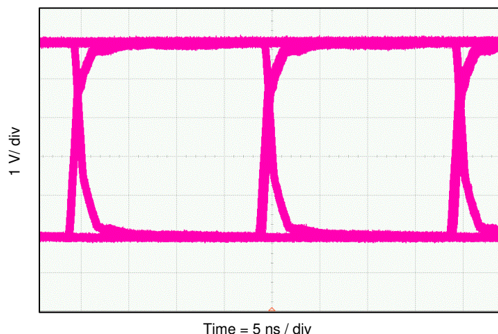
Figure 9-2. Eye Diagram at 50 Mbps PRBS 2 16 – 1, 5 V and 25°C
