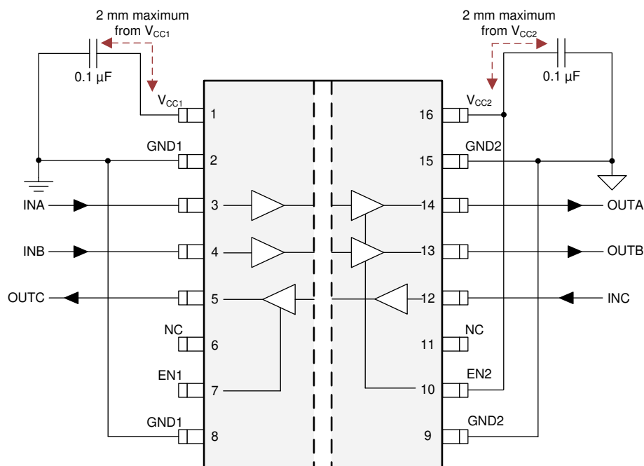
Figure 9-1. Typical ISO6731 Circuit Hook-up
