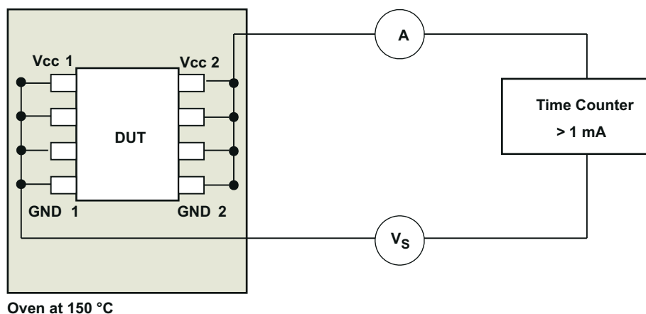
Figure 9-3. Test Setup for Insulation Lifetime Measurement
