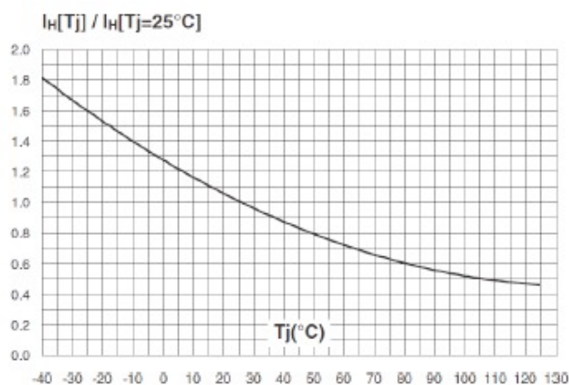
FIG.5- RELATIVE VARIATION OF HOLDING CURRENT VERSUS JUNCTION TEMPERATURE
