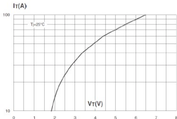
FIG.2- ON-STATE CURRENT VERSUS ON-STATE VOLTAGE (TYPICAL VALUES)
