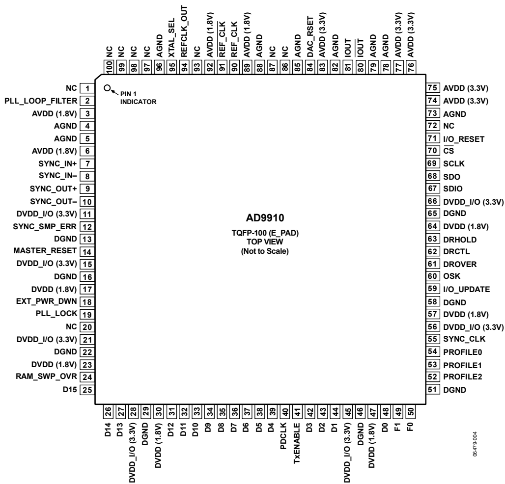
Figure 5. Pin Configuration
