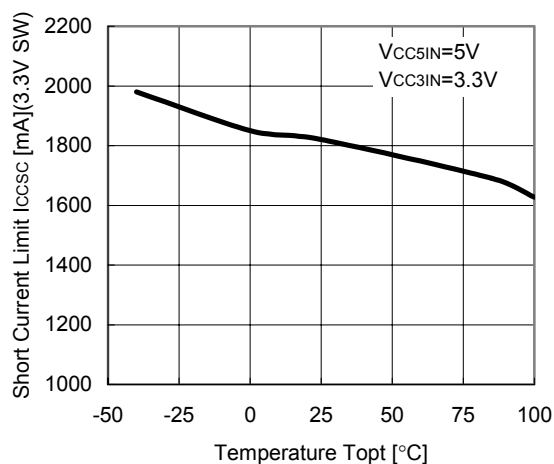
6) Short Current Limit vs. Temperature (Select VCCOUT=3.3V)
