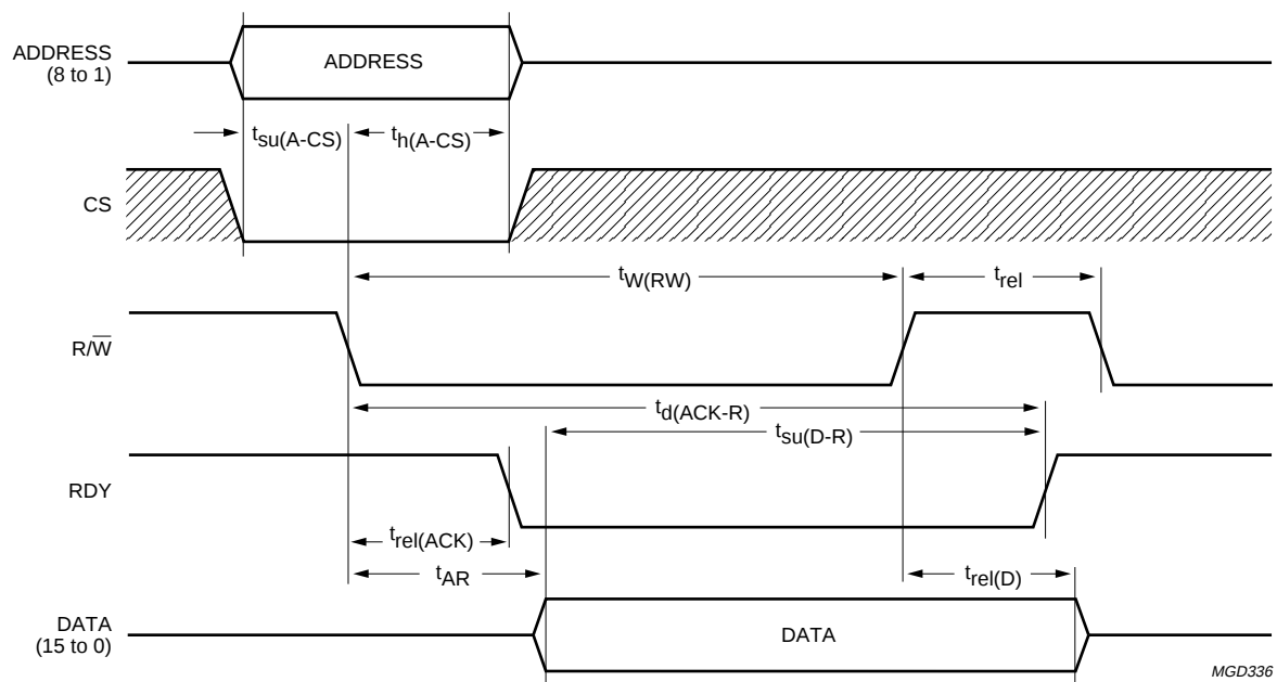
Fig.16 Intel read timing (non-multiplexed).
