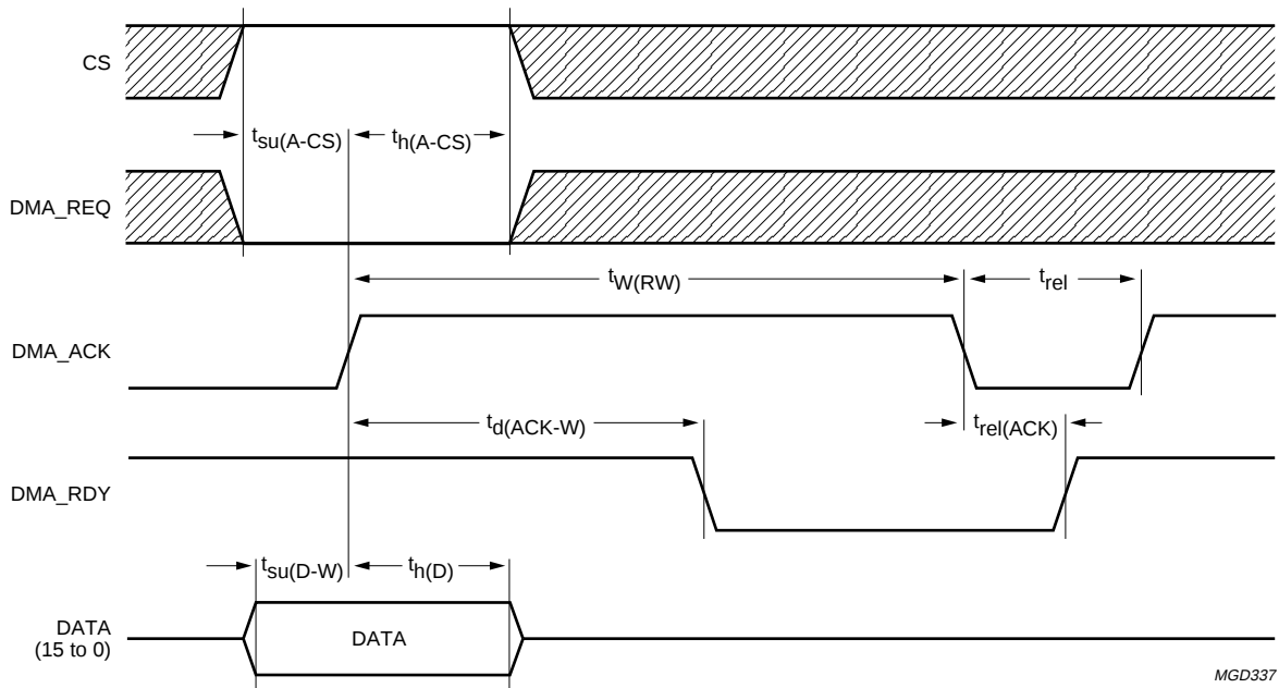
Fig.17 DMA read access.
