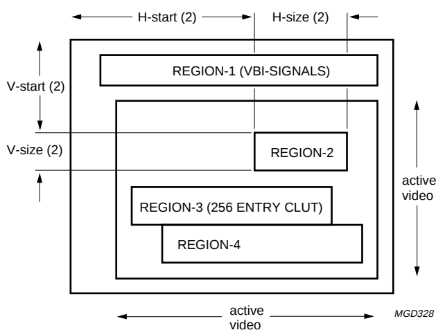
Fig.8 Graphics unit.
