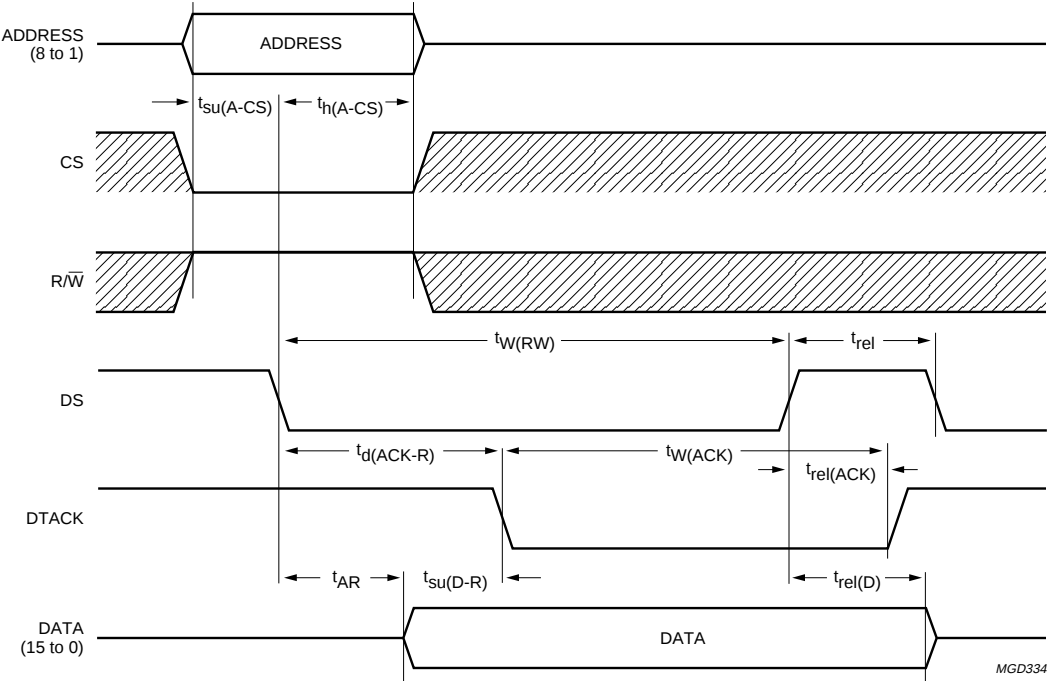
Fig.14 Motorola read timing (non-multiplexed).
