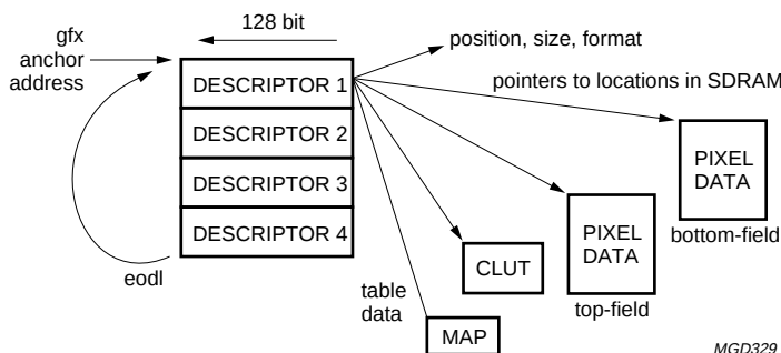
Fig.9 Display list.
