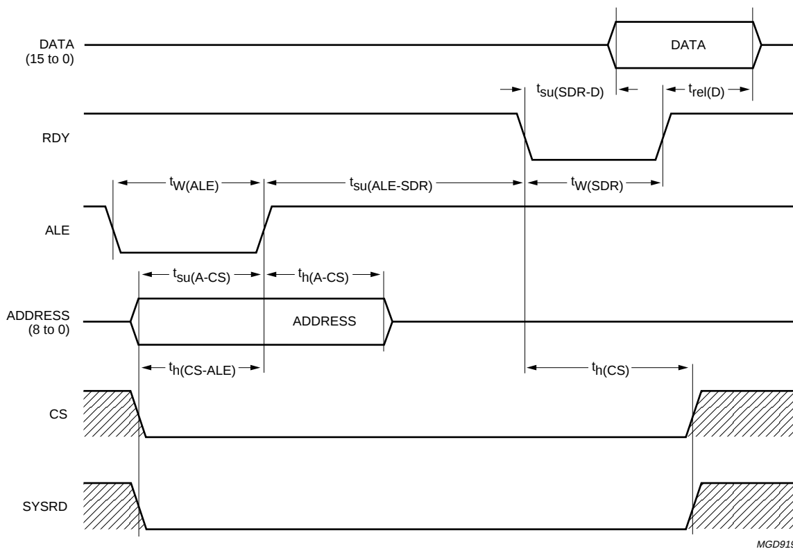
Fig.20 SAA7208 mode; read timing.
