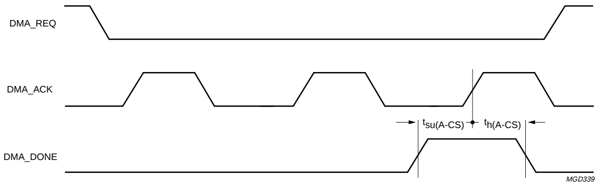
Fig.19 DMA_DONE timing.
