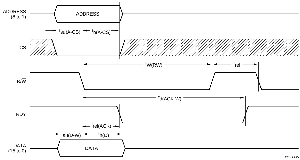
Fig.15 Intel write timing (non-multiplexed).
