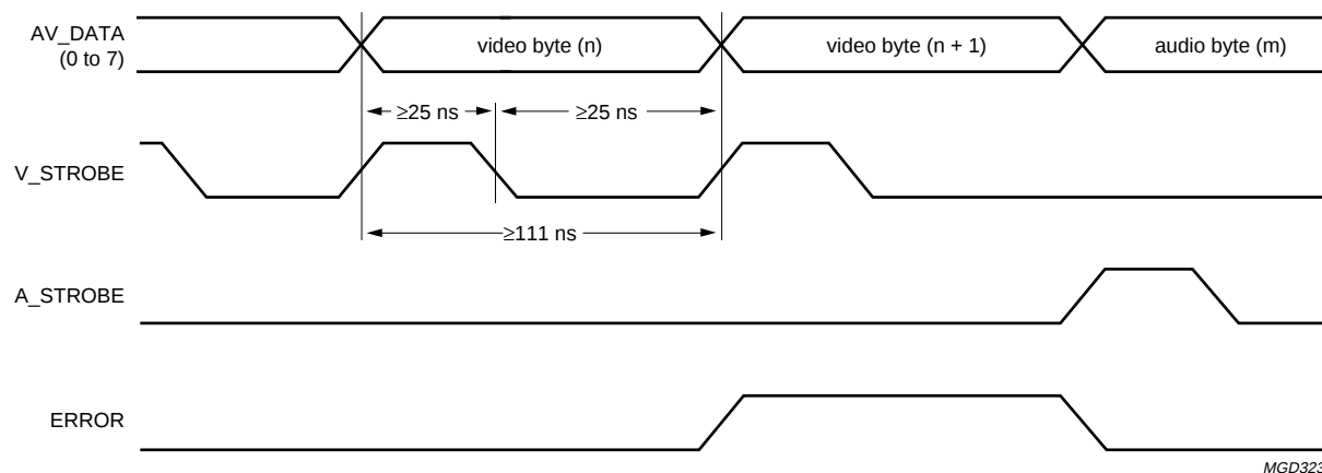
Fig.3 Timing diagram of parallel input mode.
