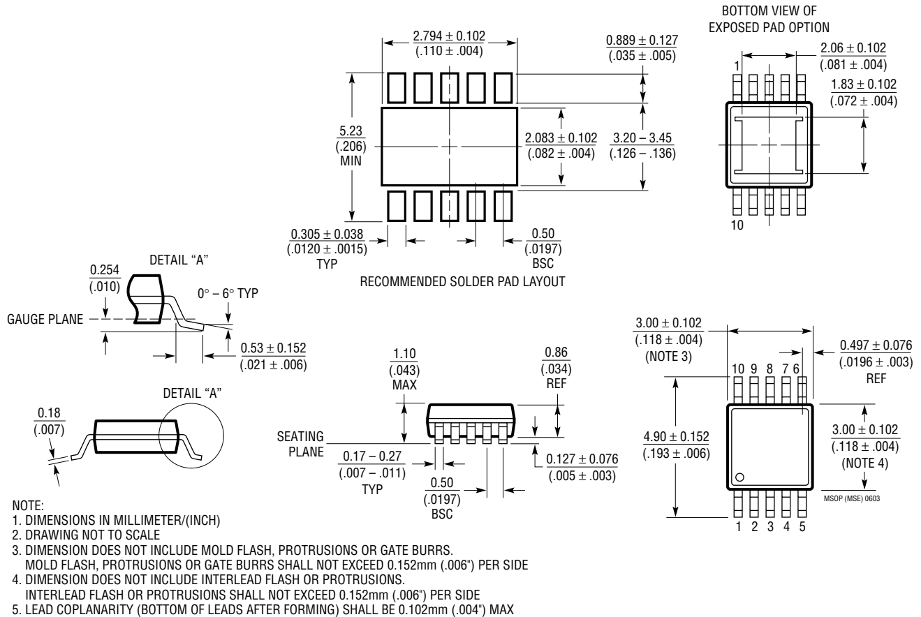
MSE Package 10-Lead Plastic MSOP (Reference LTC DWG # 05-08-1663)
