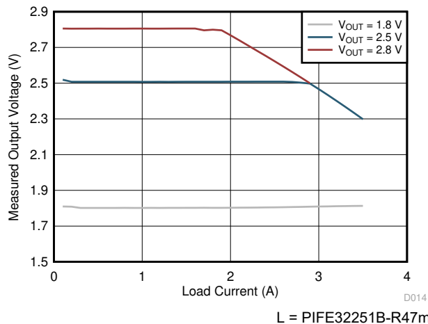
图 7-7. Converter Load Current Limitations with V_{IN} = 3.3\text{ V}
