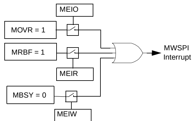
Figure 30. MWSPI Interrupts
