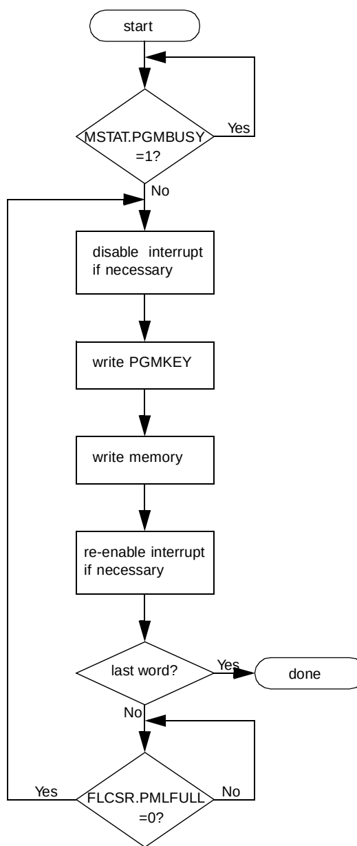
Figure 2. Programming Sequence for the Program Memory
