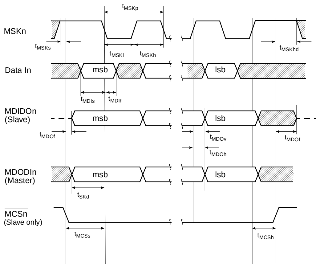
Figure 86. MICROWIRE Transaction Timing, Alternate Mode, MIDL bit = 1
