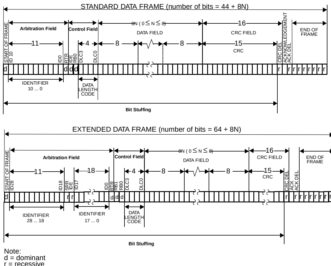
Figure 46. CAN Data Frame (standard and extended)
