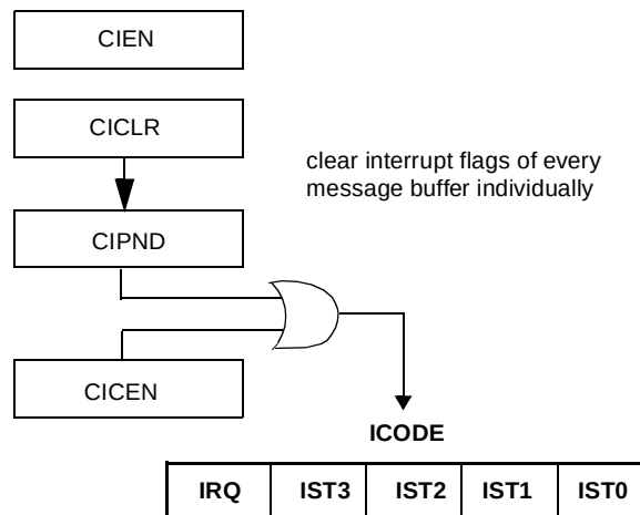
Figure 67. CR16CAN Interrupt Management
