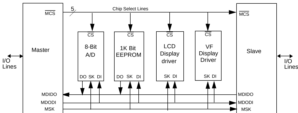
Figure 24. MICROWIRE Interface
