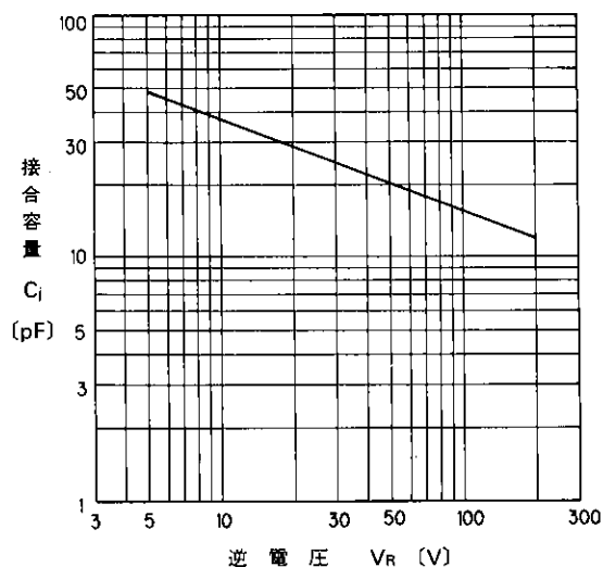
Junction Capacitance
