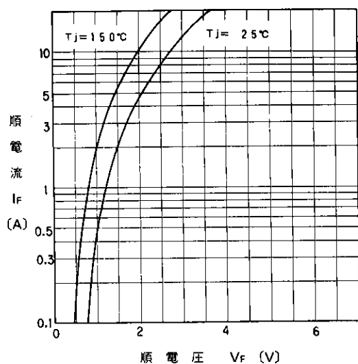
Forward Characteristics
