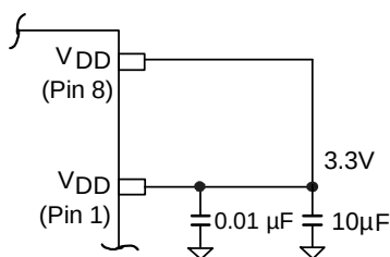
Figure 8. Power Supply Filtering
