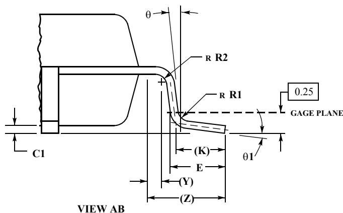
Figure 21. 112-Pin LQFP Mechanical Dimensions (Case No. 987)
