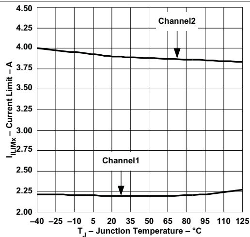
Figure 8. Current Limit vs Temperature
