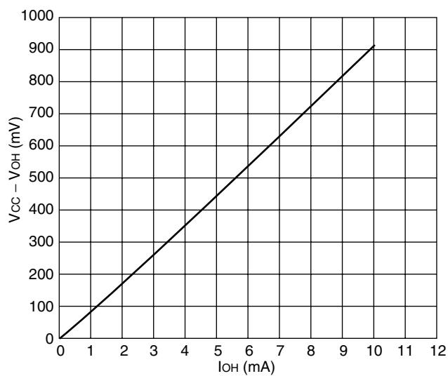
Example MB90523A V_{OH} - I_{OH} Characteristics Ta = +25 °C, V_{CC} = 4.5 V
