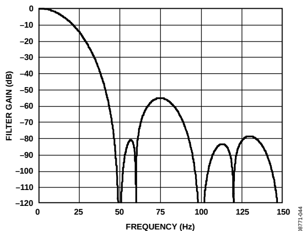
图31. \text{Sinc}^4 滤波器响应( \text{FS}[9:0] = 96 , \text{REJ}60 = 1 )
