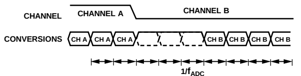
图33. \text{Sinc}^3 通道切换
