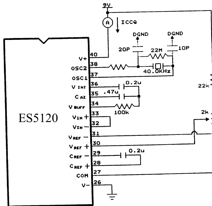
Fig.4 ICCQ Test Circuit
