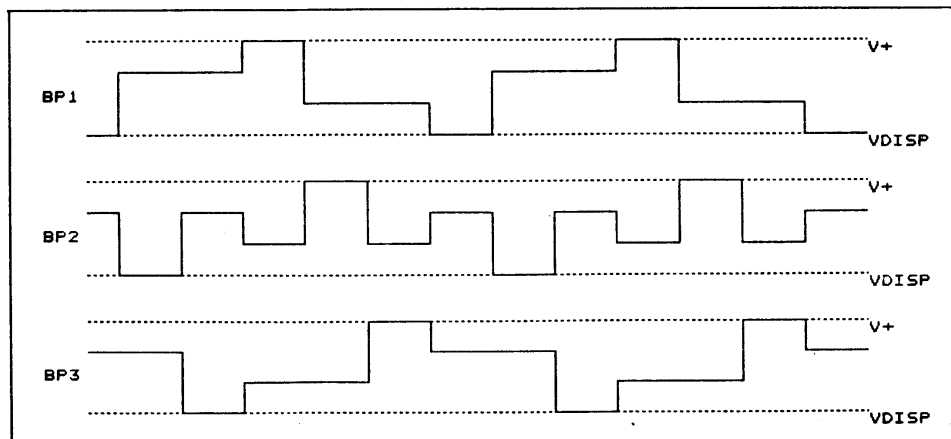
Fig.9 Backplane Waveforms
