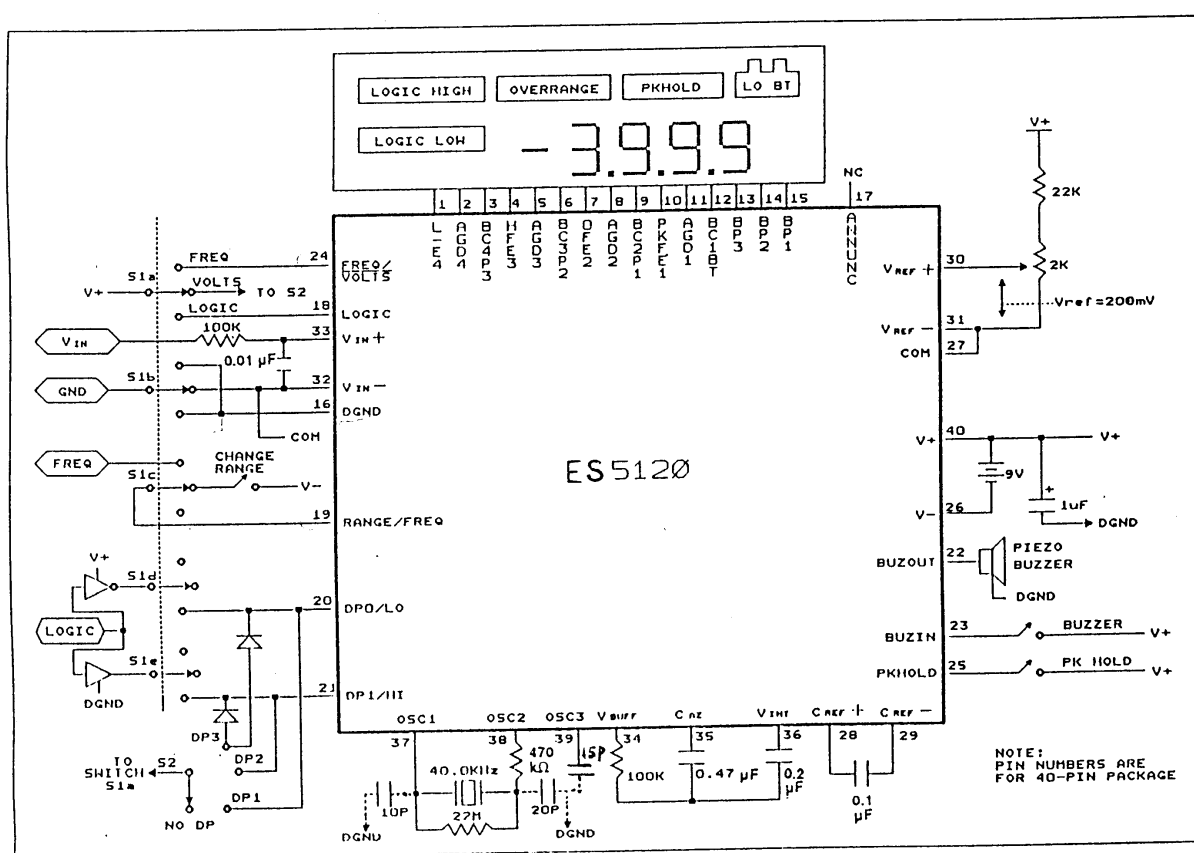
Fig. 1 Operating Circuit
