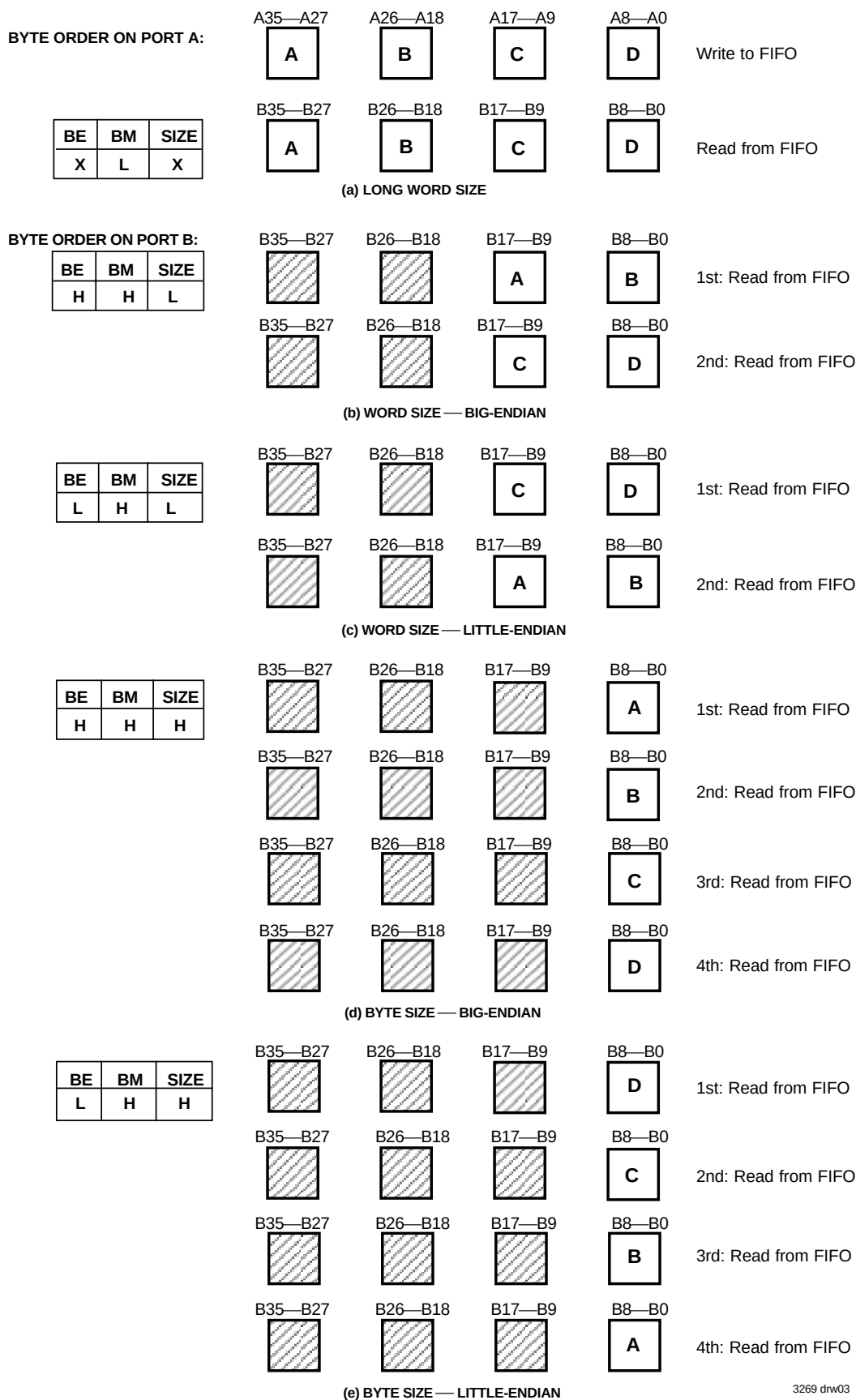
Figure 2. Bus sizing
