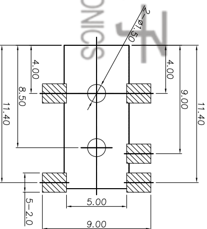
RECOMMENDED PCB LAYOUT TOP VIEW (TOLERANCE:±0.05)
