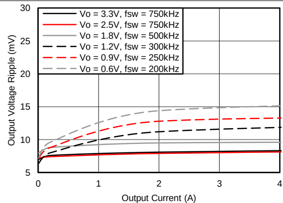
Figure 7. Voltage Ripple vs. Output Current
