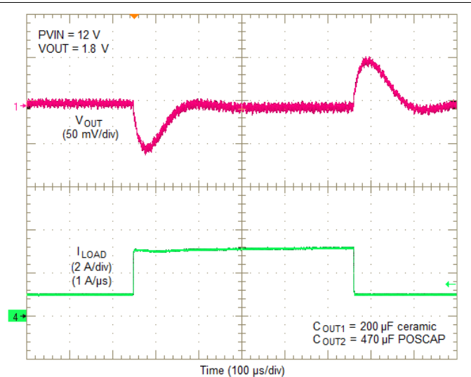
Figure 17. PVIN = 12V, VOUT = 1.8V, 2A Load Step
