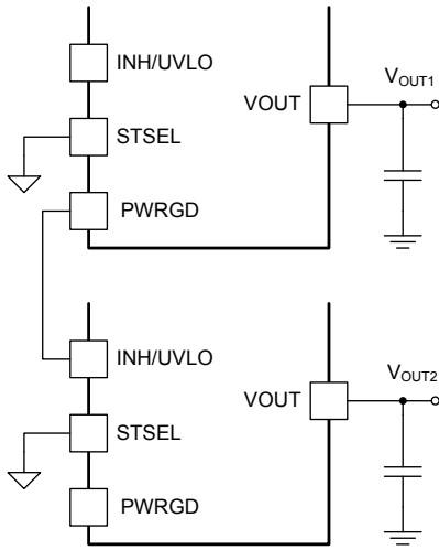
Figure 35. Sequencing Schematic
