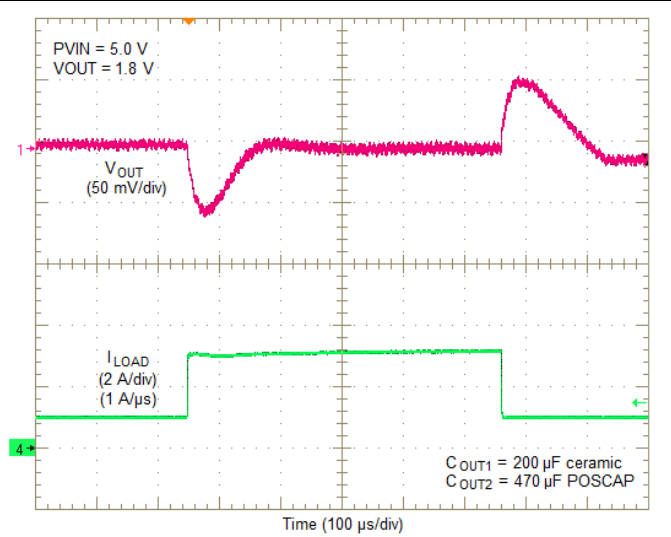
Figure 19. PVIN = 5V, VOUT = 1.8V, 2A Load Step
