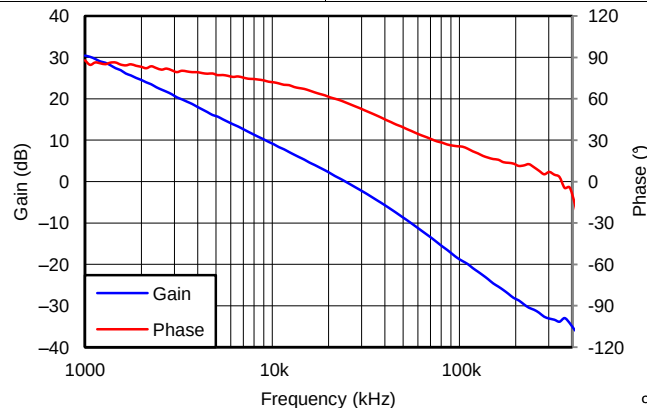
Figure 15. V OUT = 1.8 V, I OUT = 4 A, C OUT = 200 µF ceramic, f sw = 500 kHz
