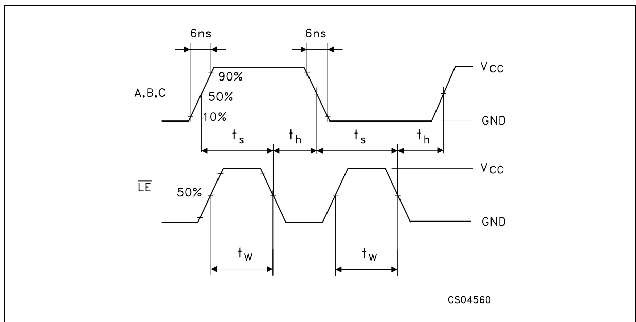
WAVEFORM 2 : MINIMUM PULSE WIDTH, SETUP AND HOLD TIME ( f=1\text{MHz} ; 50% duty cycle)
