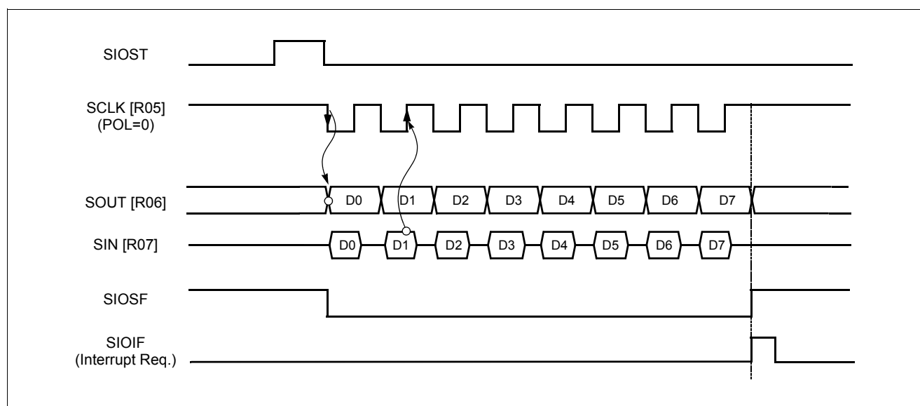
Figure 15-3 SPI Timing Diagram at POL=0
