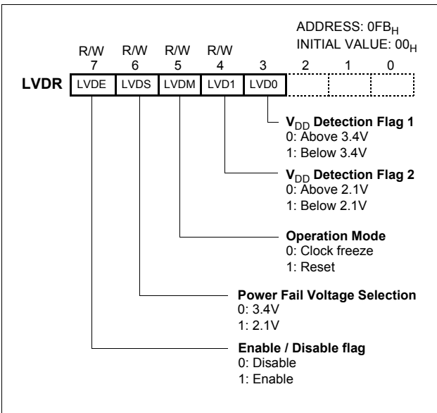
Figure 23-1 Low Voltage Detector Register
