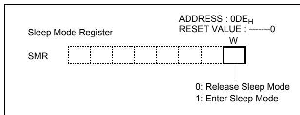
Figure 20-1 SLEEP Mode Register
