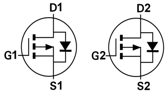
Equivalent Circuit
