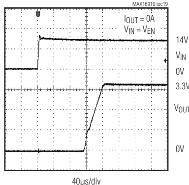
POWER-UP RESPONSE
