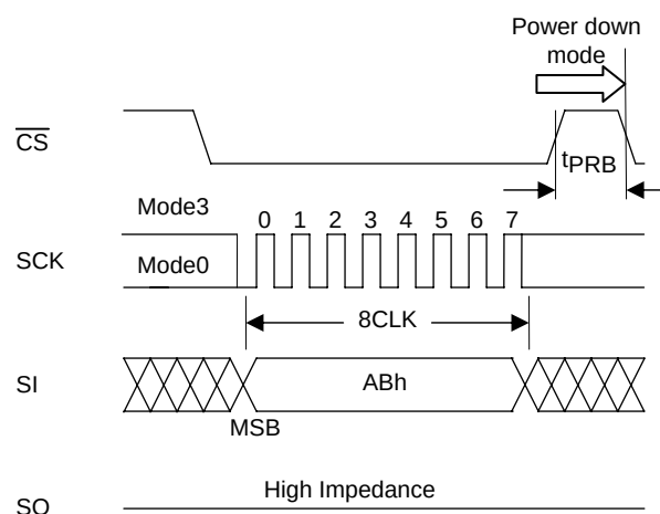
Figure 11 Exiting from Power-down
