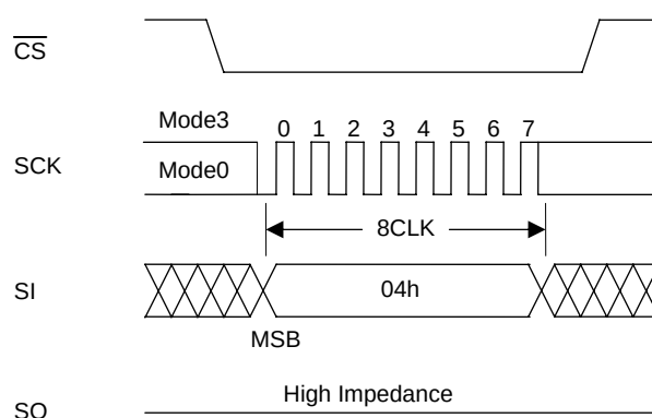
Figure 9 Write Disable
