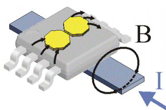
Figure 1: Typical application of MLX91208
