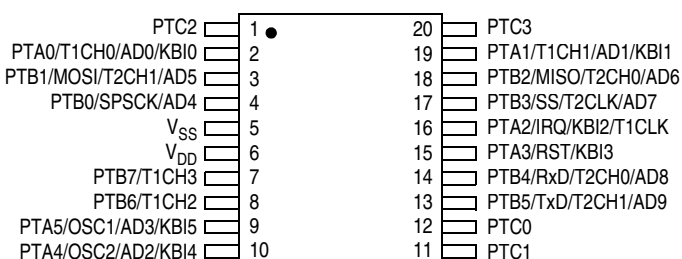
20-PIN ASSIGNMENT MC68HC908QCxx TSSOP
