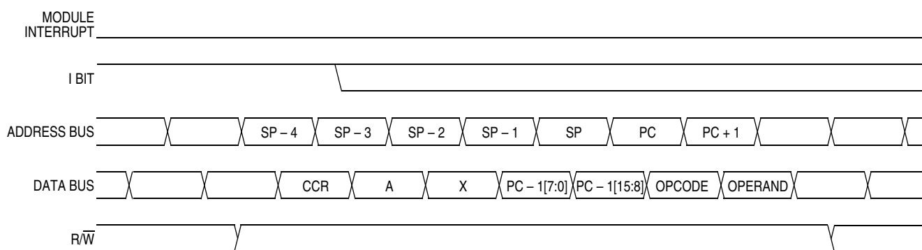
Figure 14-9. Interrupt Recovery
