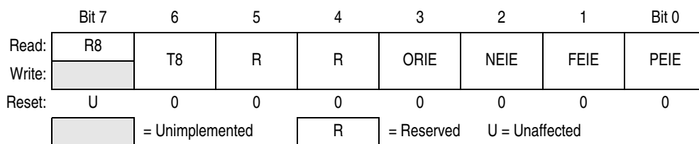
Figure 13-11. ESCI Control Register 3 (SCC3)
