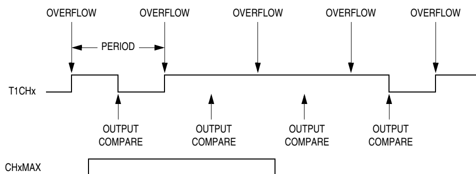
Figure 16-13. CHxMAX Latency
