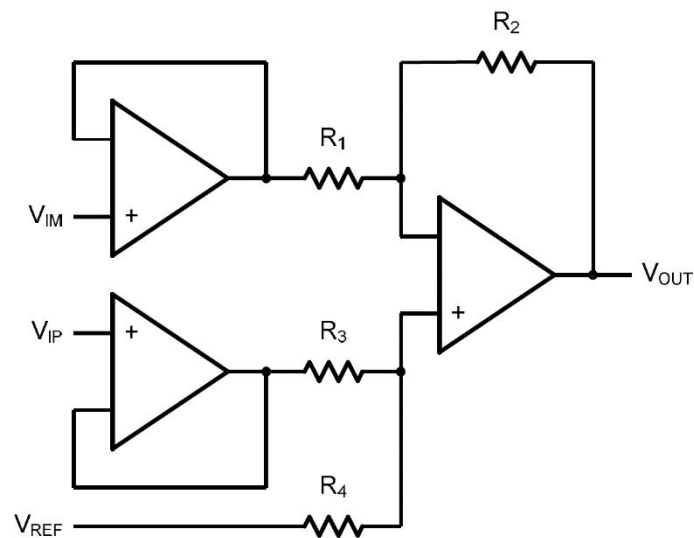
Figure 6. Instrument Amplifier
