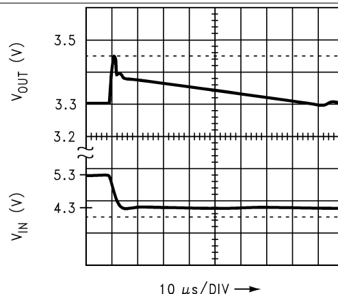
Figure 16. Line Transient Response
