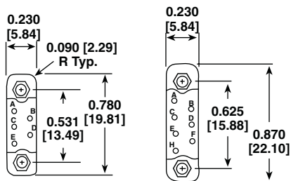
5 CONTACTS
