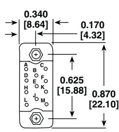
11 CONTACTS
