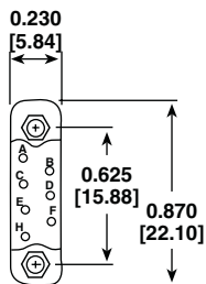
7 CONTACTS
