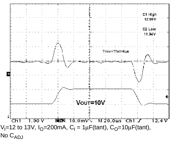
Figure 26: Line Transient
