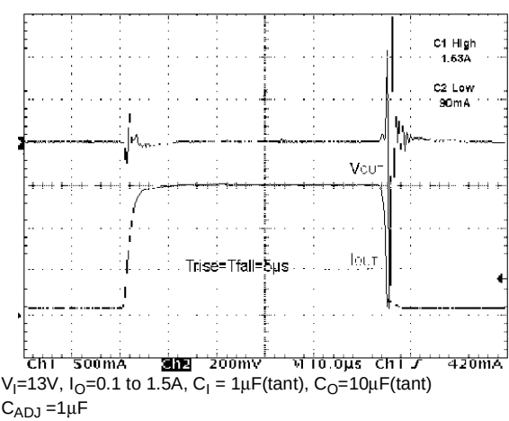
Figure 27: Load Transient
