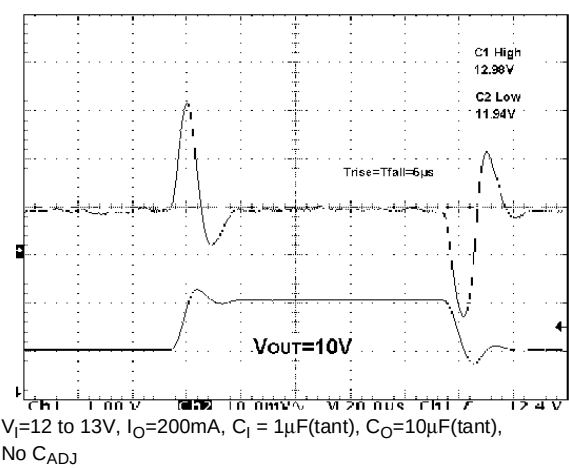
Figure 24: Line Transient
